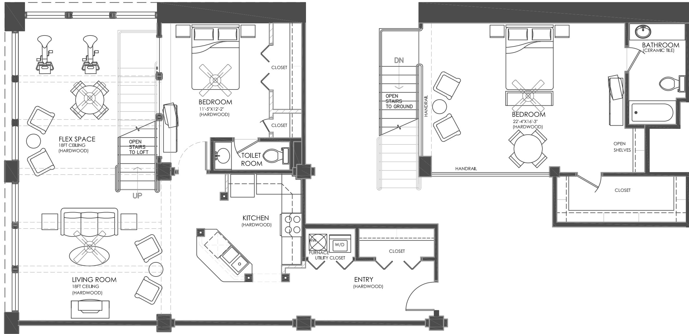
UNIT 1A (1078 SF) (1502 SF) TOTAL HEATED AREA
